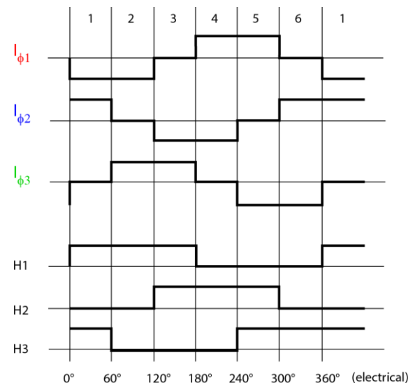
Figure 8: Output from the Hall-effect sensors on a three-phase motor (H1, H2, and H3) enables the drive to determine rotor position and properly generate drive currents for the three windings ( I_{\phi 1} (red), I_{\phi 2} (blue), and I_{\phi 3} (green)). This commutation diagram shows the six current levels that give six-step commutation its name.
