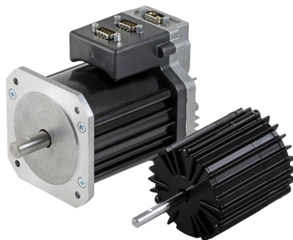
Figure 15: Examples of BLDC motors with (left, EnduraMax 95i ) and without (right, EnduraMax 75n ) integrated control electronics.
